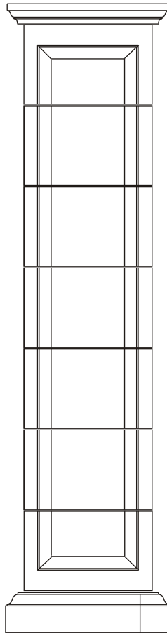
Gate Pier GP10 Including Pier cap (PCD24) Height 2,340 (including 12mm of grouting) £660.95 597kg Extra 300mm of shaft (GP13): £72.60 Core: minimum 320mm square.
