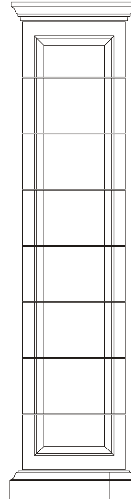
Gate Pier GP20 Including Pier cap (PCD27) Height 2,666 (including 12mm of grouting) £860.40 900kg Extra 300mm of shaft (GP23): £84.70 Core: minimum 359mm square.
