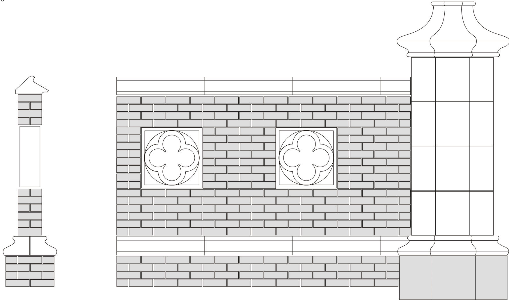
Gothic Wall. Wall Coping WCG1, with Wall Plinth WP11 and Quatrefoils BS31 Approximately £197.80 per metre. Please call for a quotation Illustrated with Gate Pier GP80 See page 4.15
