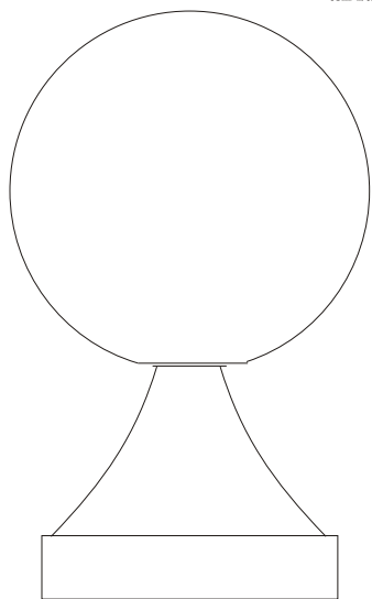
Sloping base F093 Base width 356mm Base height 279mm £22.13 28Kg
