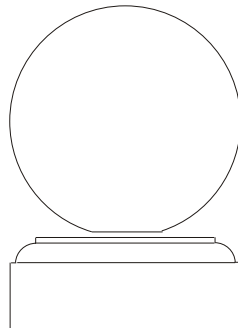
Plinth UP06P Plinth width 303mm Plinth height 122mm £21.28 20Kg
