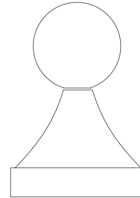
Sloping base F093 Base width 356mm Base height 279mm £22.13 28Kg
