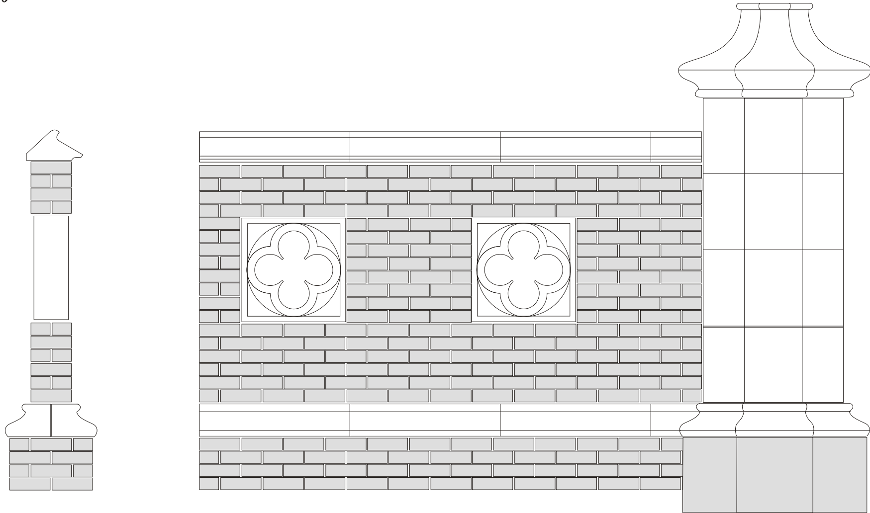
Gothic Wall. Wall Coping WCG1, with Wall Plinth WP11 and Quatrefoils BS31 Approximately £172 per metre. Illustrated with Gate Pier GP80 See page 4.15
