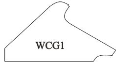
Wall coping WCG1 £49.50/m 46Kg/m Max. width 300mm, wall width 240mm Height 162mm See also page 4.21
