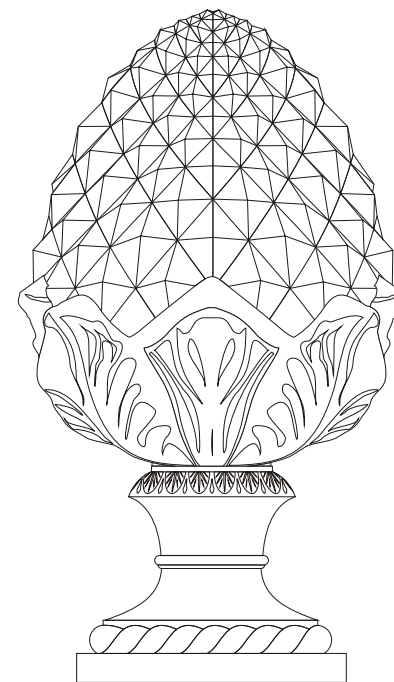
Pineapple and Base F002 £161.70 104Kg Overall height 889mm Base width 330mm Maximum width 508mm
