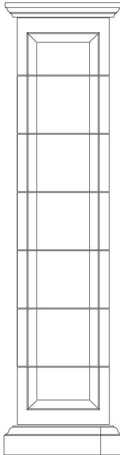
Gate Pier GP10 Including Pier cap (PCD24) Height 2,340 (including 12mm of grouting) £605.00 597 Kg Extra 300mm of shaft (GP13): £66.00 Core: minimum 320mm square.
